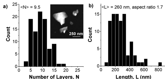
Figure 2. a) Thickness and b) length histograms compiled from atomic force microscopy after drop-casting a 2H-MoS 2 dispersion onto Si/SiO 2 wafers. Inset in (a): representative AFM image.
